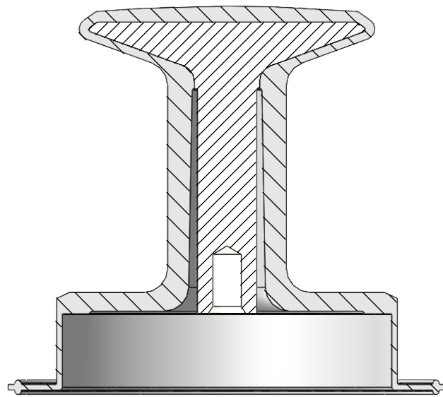
SECTION VIEW
